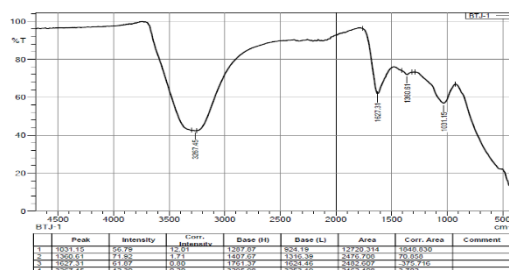
Gambar 5. FTIR Biochar tongkol jagung
